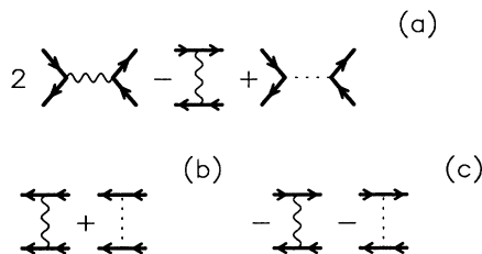
FIG. 1. Lowest-order contribution to the irreducible vertex function in the (a) charge-density-wave, (b) superconducting, and (c) spin-density-wave channels. The solid lines denote electron propagators, the wiggly lines denote phonon propagators, and the dotted lines denote the Coulomb repulsion.
