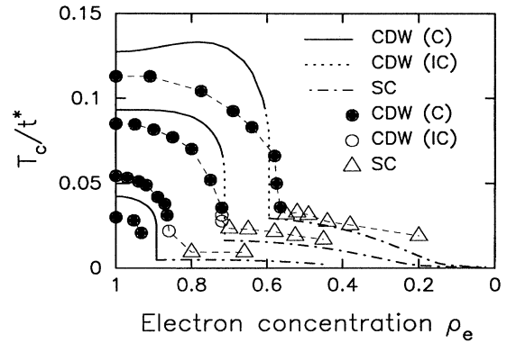
FIG. 2. Phase diagram for the Holstein-Hubbard model with g = 0.5 , \Omega = 0.5 , U = -1.0 , and U_C = 0.0, 0.25, 0.5 , and 0.75 . The solid dots (lines) are for the commensurate CDW, the open dots (dotted lines) are for the incommensurate CDW, and the open triangles (dot-dashed lines) are for the SC as determined from a QMC (IPT) calculation. There are no transitions detected by the IPT for U_C = 0.75 . The dashed line through the QMC points is a guide to the eye.
