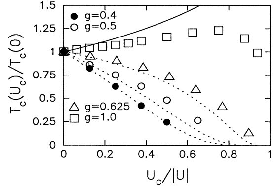
FIG. 3. Relative change in the CDW transition temperature at half filling due to Coulomb repulsion. Four different cases are shown: g = 0.4 (solid dots), g = 0.5 (open dots), g = 0.625 (open triangles), and g = 1.0 (open squares). The dotted lines are the weak-coupling approximations for g = 0.4, 0.5, and 0.625 . The parameter I is adjusted to produce the correct slope as U_C \rightarrow 0 . The solid line is a fourth-order strong-coupling approximation for the g = 1.0 case.
