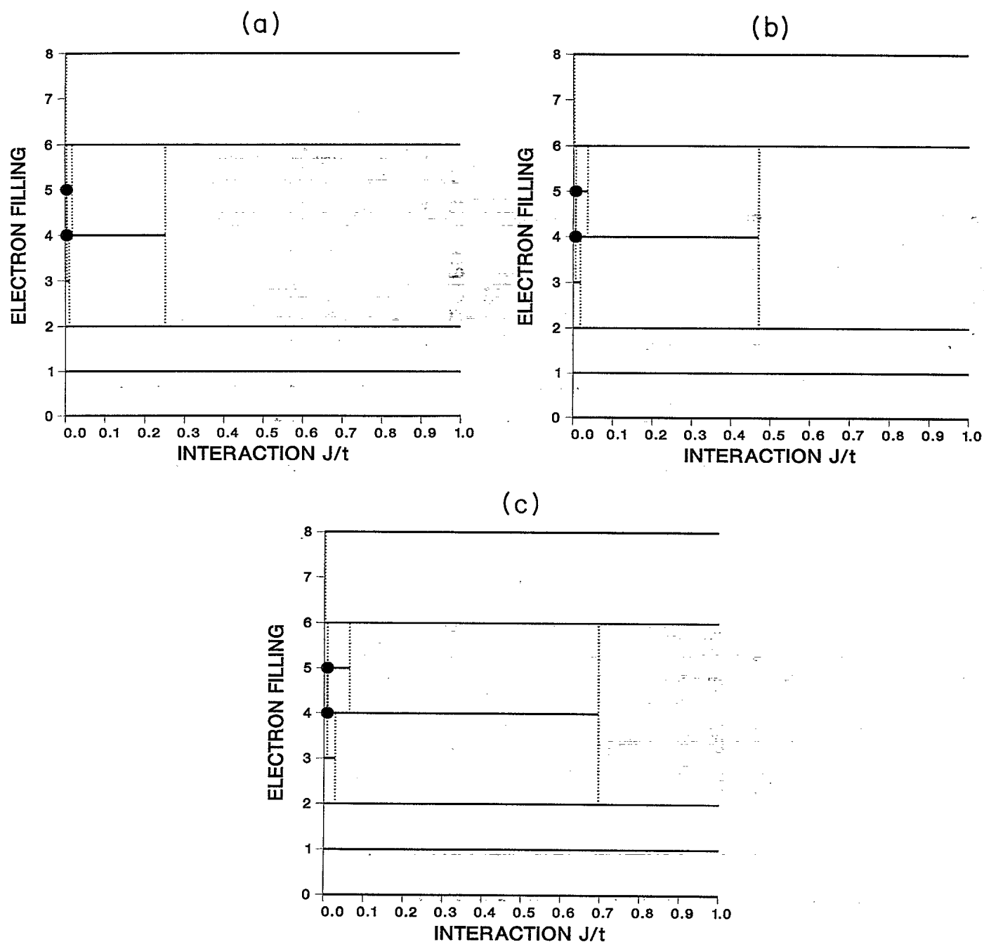
FIG. 7. Stability phase diagram for the fcc ( t > 0 ) lattice. Three cases have been calculated: (a) t' = 0.15|t| , (b) t' = 0.0 , and (c) t' = -0.15|t| .
