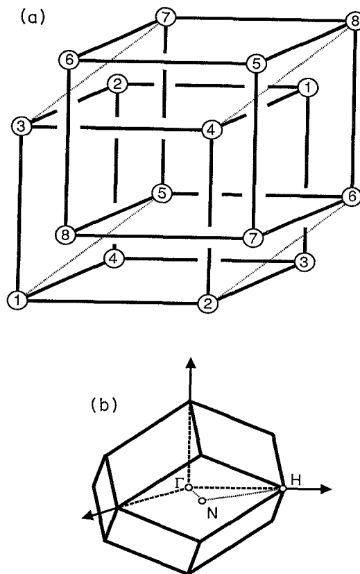
FIG. 2. Eight-site cluster with PBC's for the bcc lattice in (a) real and (b) reciprocal space. The dotted line in (a) is the body diagonal. The nearest neighbors of site 5 are two each of sites 1, 2, 3, and 4. The three symmetry stars in (b) are \Gamma = (0,0,0) , H = (2,0,0)\pi/a , and N = (1,1,0)\pi/a .
