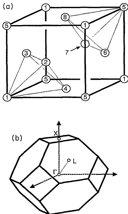
FIG. 3. Eight-site cluster with PBC's for the fcc lattice in (a) real and (b) reciprocal space. The double-tetrahedral structure is highlighted with dotted lines in (a). The three symmetry stars in (b) are \Gamma = (0,0,0) , X = (0,0,2)\pi/a , and L = (1,1,1)\pi/a .
