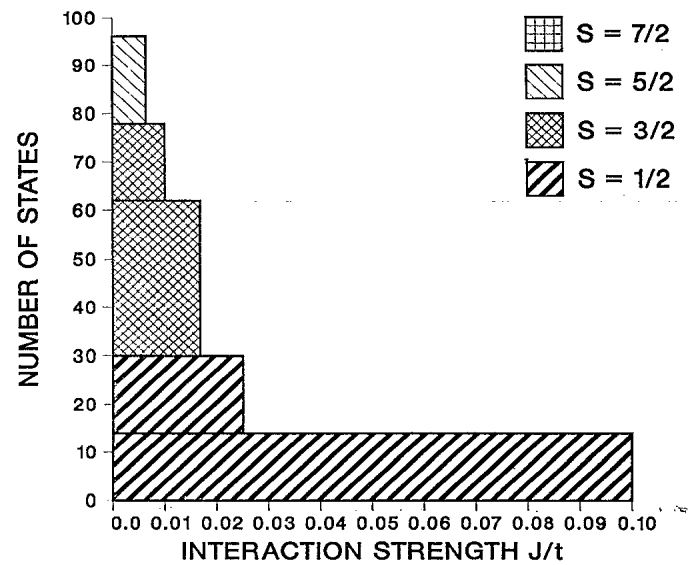
FIG. 11. Total number of states in the ground-state manifold and in the low-lying excitations within 0.1|t| of it for the fcc ( t > 0 ) lattice and N=7 . There are no low-lying excitations in the range 0.1 < J/t < 1.0 . The spin-pileup effect can be seen at J=0 .
