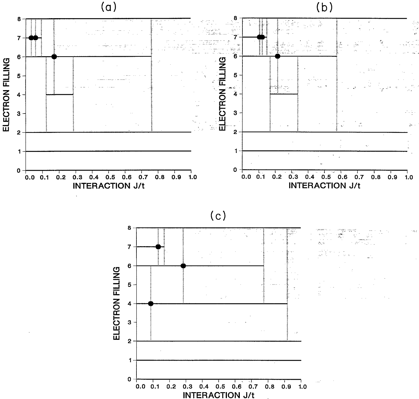
FIG. 9. Stability phase diagram for the sq lattice. Three cases have been calculated: (a) t'=0.15|t| , (b) t'=0.0 , and (c) t'=-0.15|t| . Note the phase islands for N=4 .
