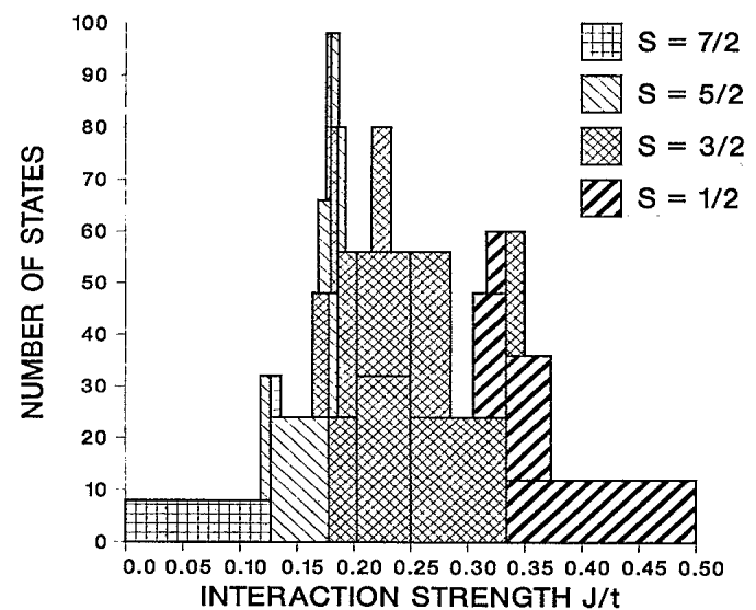
FIG. 12. Total number of states in the ground-state manifold and in the low-lying excitations within 0.1|t| of it for the fcc ( t < 0 ) lattice with t'=0 and N=7 . There are no low-lying excitations in the range 0.5 < J/t < 1.0 .
