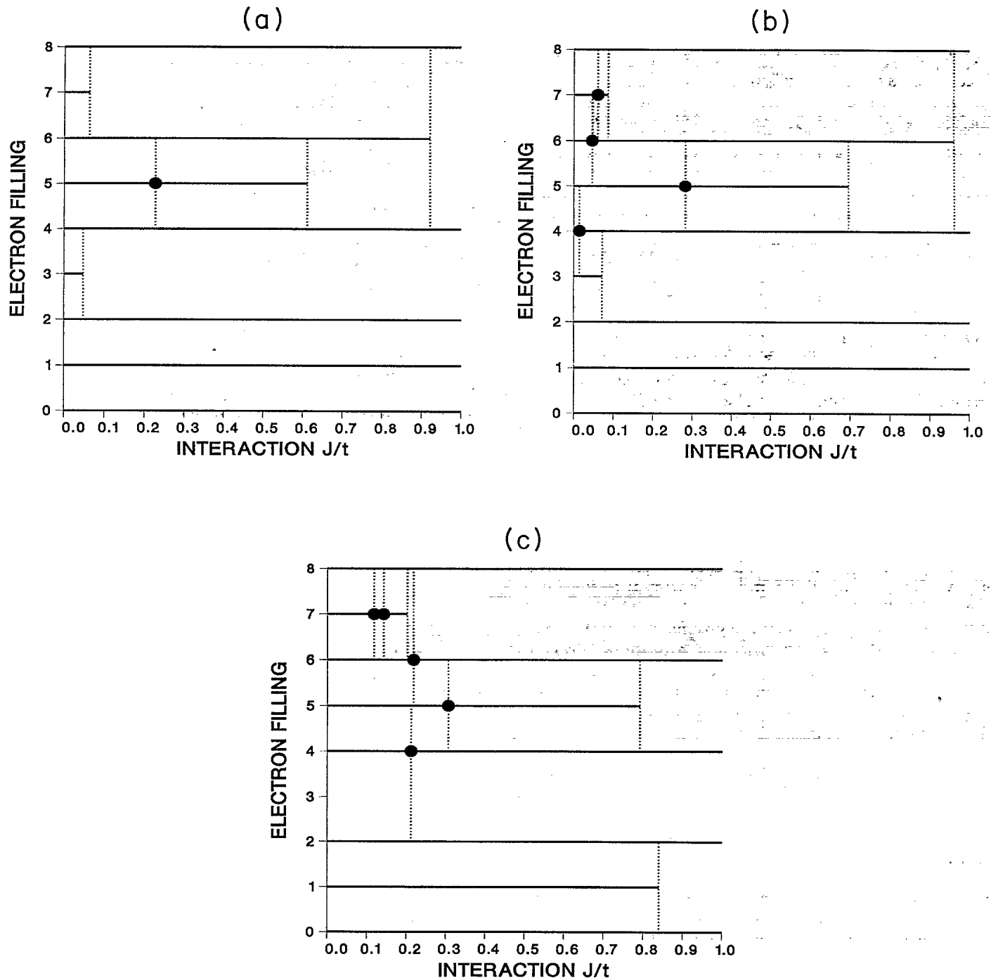
FIG. 5. Stability phase diagram for the sc lattice. The x axis is the interaction strength J/t and the y axis is the electron filling N . Solid horizontal lines correspond to stable single phases. Dotted vertical lines denote discommensuration instabilities or level crossings in the fixed- N solutions. Level crossings are also marked by a black dot. Three cases have been calculated: (a) t' = 0.15|t| , (b) t' = 0.0 , and (c) t' = -0.15|t| .
