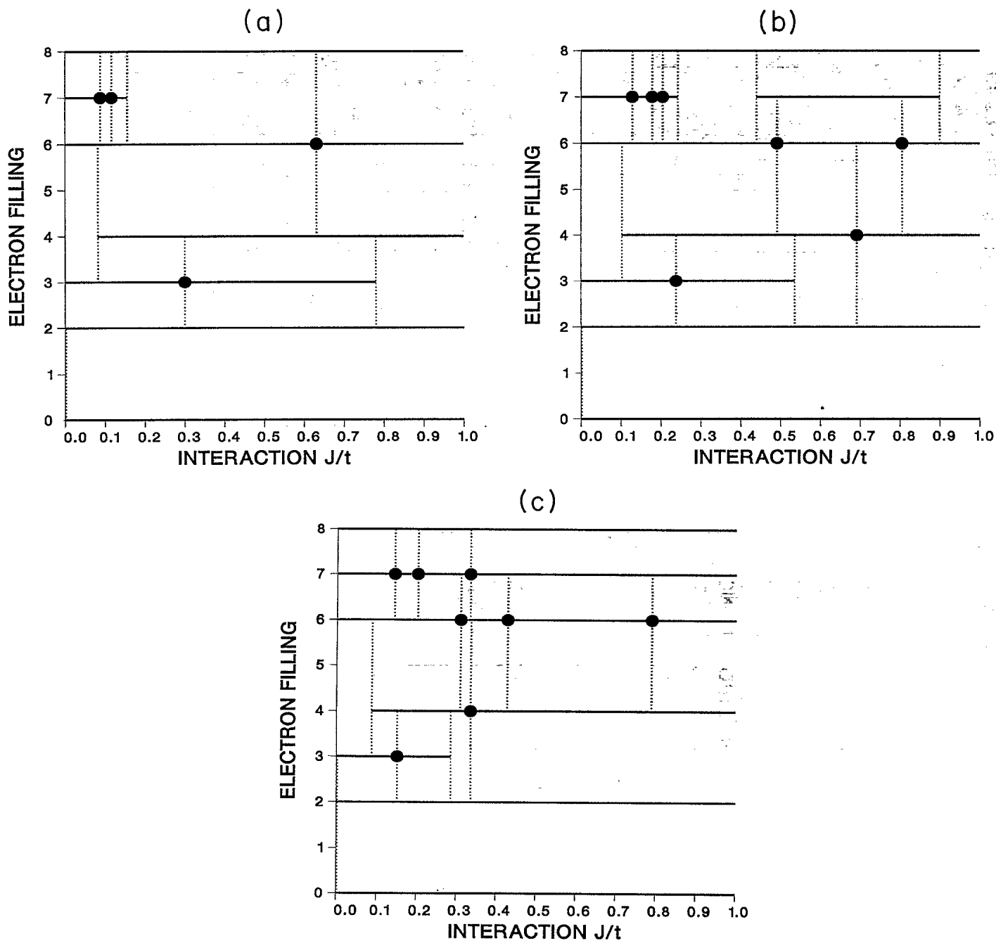
FIG. 8. Stability phase diagram for the fcc ( t < 0 ) lattice. Three cases have been calculated: (a) t' = 0.15|t| , (b) t' = 0.0 , and (c) t' = -0.15|t| . Note the phase islands for N=4 and 7 and that N=1 is unstable.
