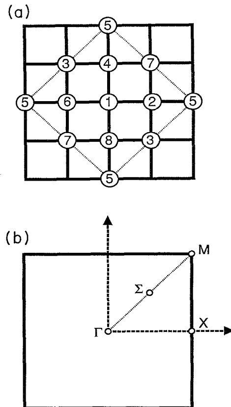
FIG. 4. Eight-site cluster with PBC's for the sq lattice in (a) real and (b) reciprocal space. The 2\sqrt{2}a \times 2\sqrt{2}a "primitive" cell is highlighted with dotted lines in (a). The four symmetry stars are \Gamma = (0,0) , M = (1,1)\pi/a , X = (1,0)\pi/a , and \Sigma = (1,1)\pi/2a .
