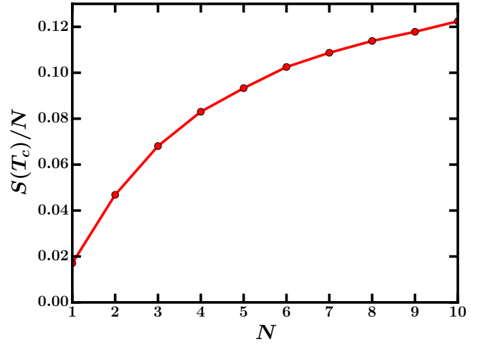
FIG. 3. The entropy of the mobile fermions S_{\text{mob}}(T_c)/N per mobile fermion at the critical temperature T_c calculated in DMFT as a function of the mobile fermion degeneracy N .
