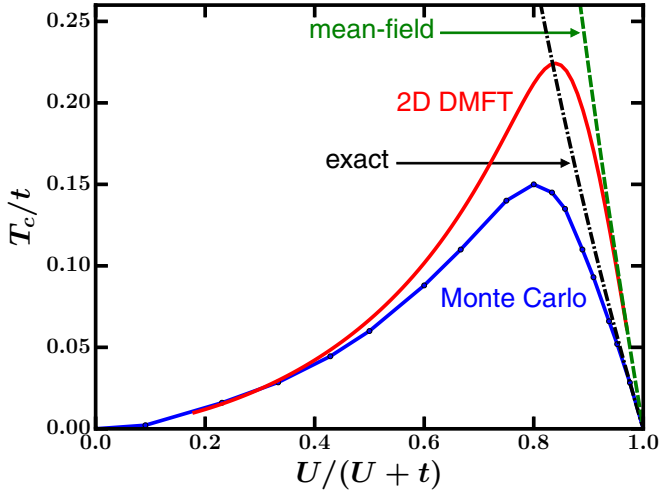
FIG. 1. Comparison of the 2D DMFT (solid red line) and MC (blue dots, connected with a solid line as a guide to the eye) critical temperatures to the checkerboard density wave at half filling for both species on a square lattice with N = 1 . The lines marked as “Ising mean-field” (green) and “Ising exact” (black) show the critical temperatures for the corresponding Ising model, which become exact for the respective theories when U \rightarrow \infty .
