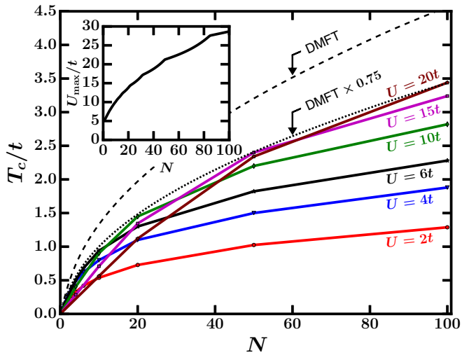
FIG. 2. The maximal critical temperature T_c plotted as a function of mobile fermion degeneracy N (as calculated with MC). The dashed line shows the corresponding DMFT T_c calculated at U = U_{\max}(\text{DMFT}) . The solid lines show MC T_c 's for different values of U . The black dotted line shows T_c(\text{DMFT}) \times 0.75 , which agrees well with nearly all the MC results. In the inset, U_{\max}(\text{DMFT}) is plotted as a function of degeneracy N , indicating it changes significantly with N .
